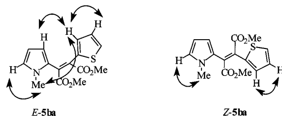
Figure 1. Selected NOE correlation of compounds E - 5ba and Z - 5ba
